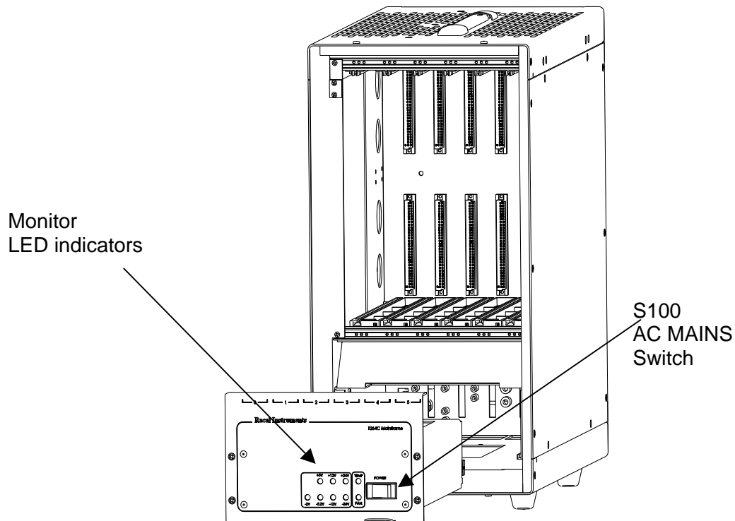
Figure 3-1, 1264C Front View
